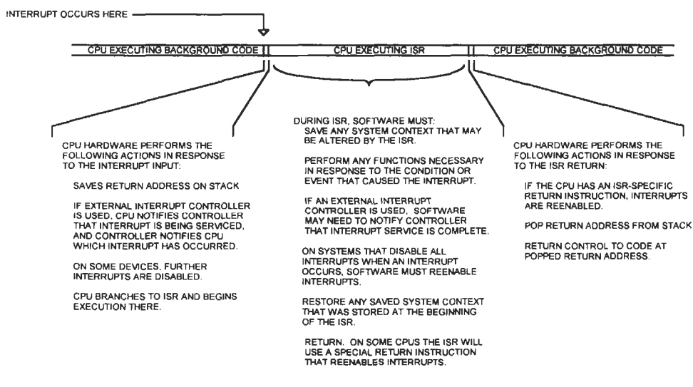
Figure 5.1 Interrupt Processing.
