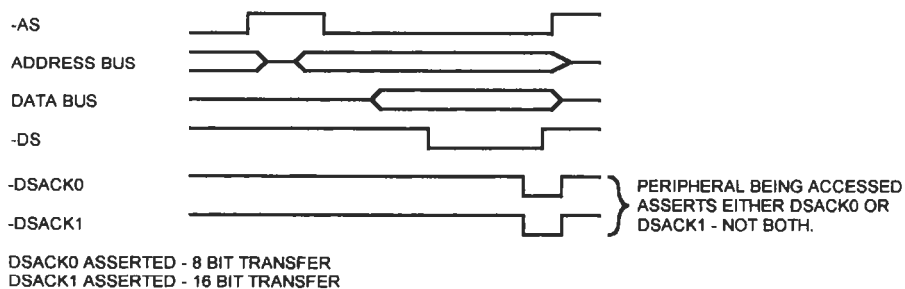
Figure 3.1 Dynamic Bus Sizing.
