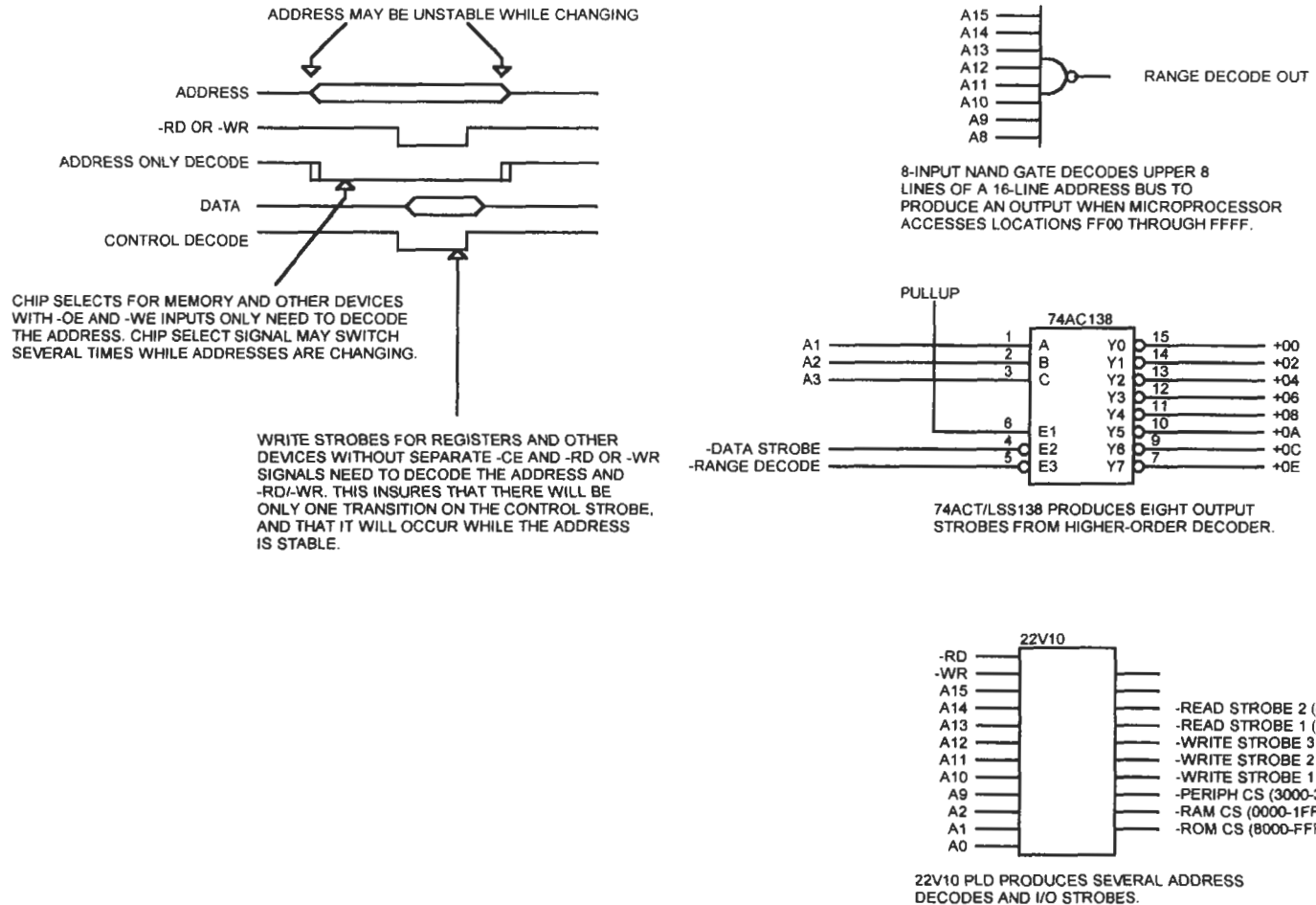
Figure 2.13 Address Decoding Circuits.
