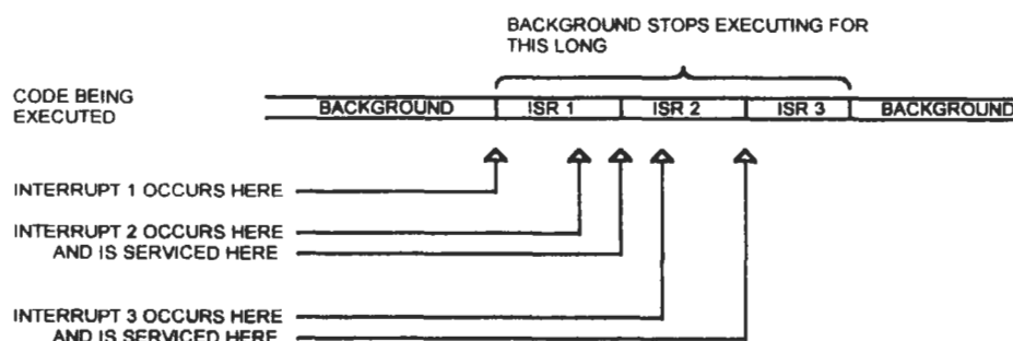
Figure 5.8 Interrupt Stackup.
