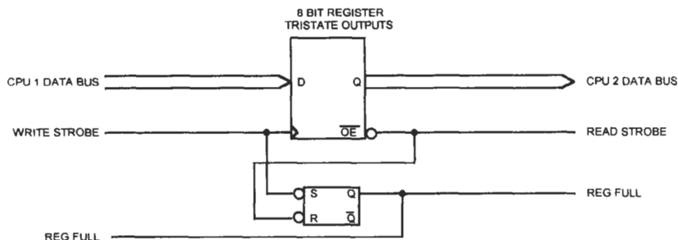
Figure 8.3 Register-Based Communication with Status Flip-Flop.
