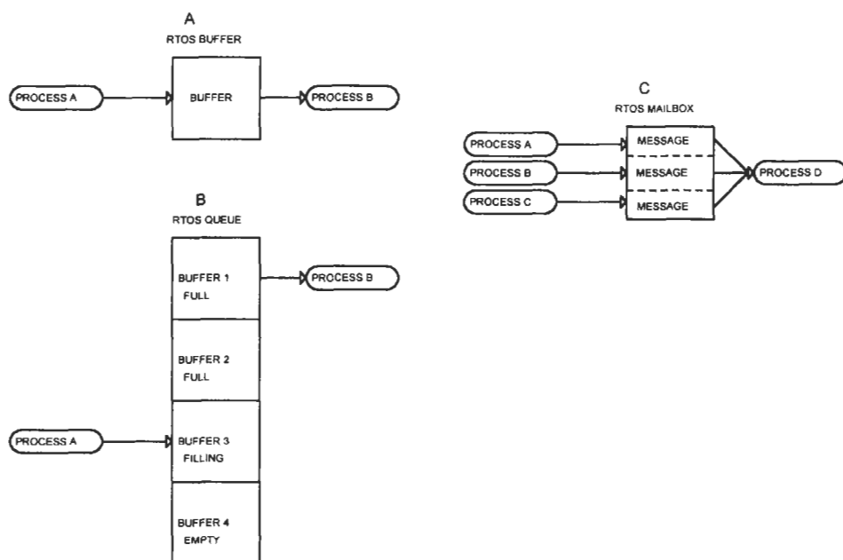
Figure 9.3 RTOS Communication.
