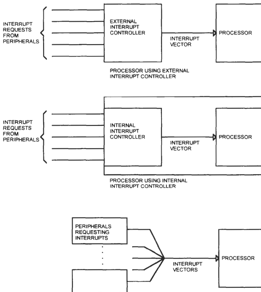
Figure 5.2 Interrupt Vector Generation.
