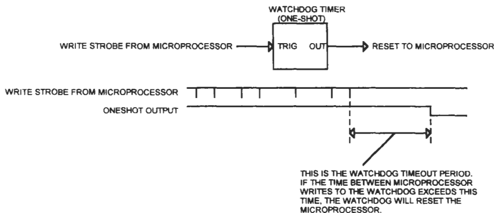
Figure 2.26 Watchdog Timing.
