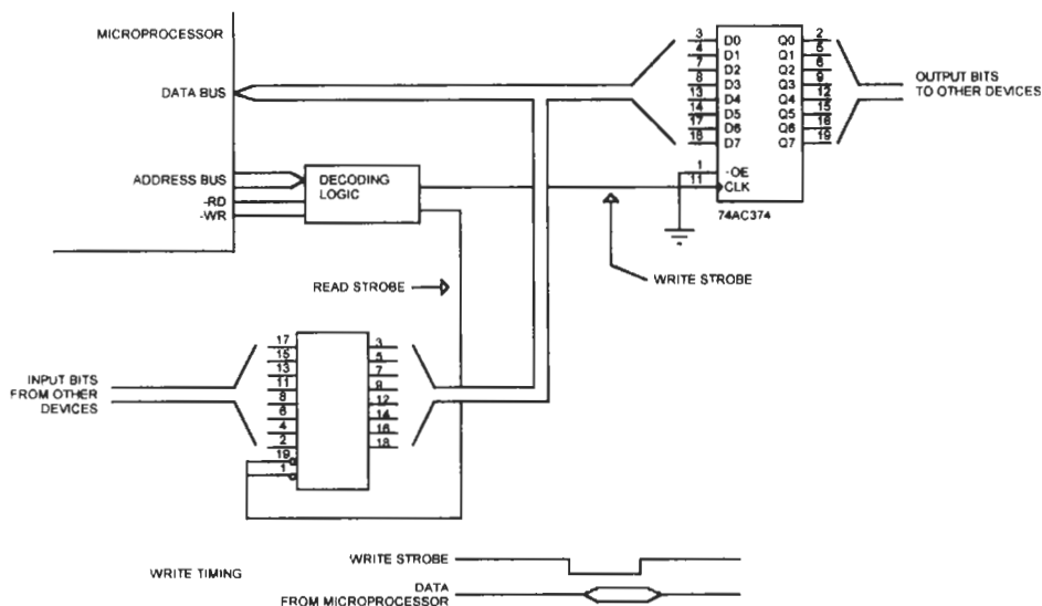
Figure 2.12 Simple Input and Output Ports.
