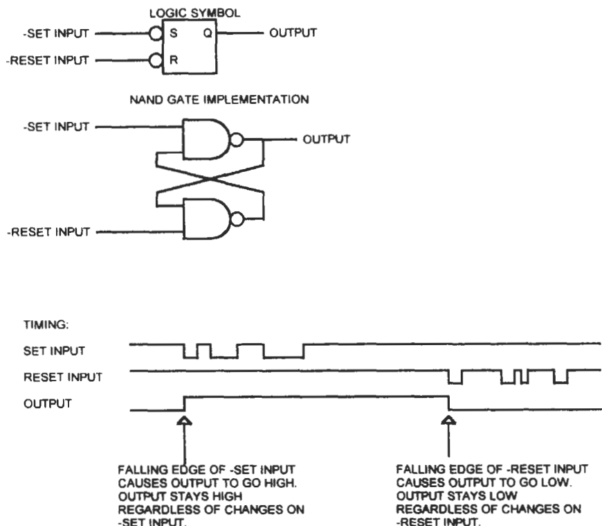
Figure C.2 Set/Reset Flip-Flop.
