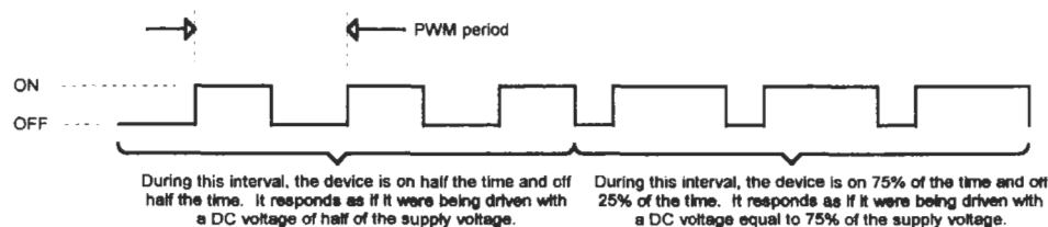
Figure 1.2 PWM Operation.
